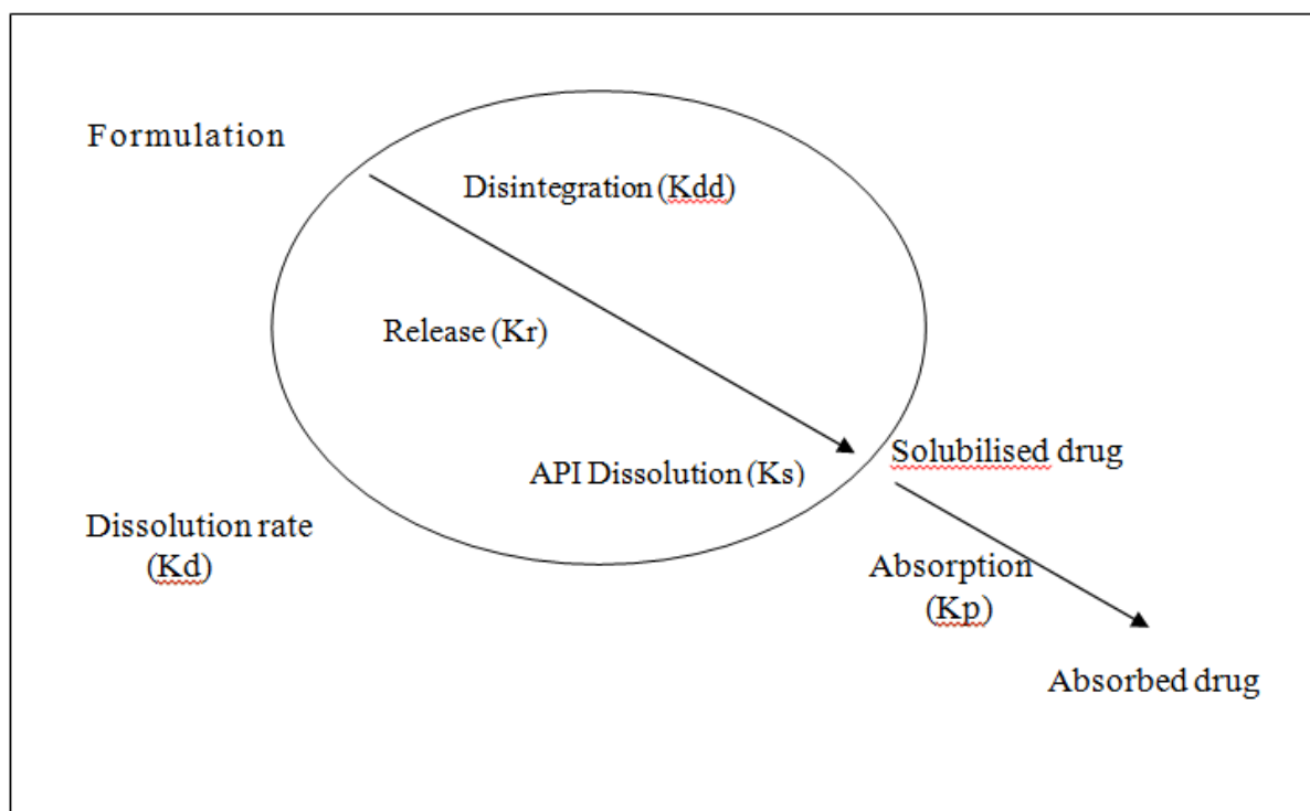
Fig. 3. Representation of the main phenomena leading to absorption in vivo , outside (macro) phenomena, inside dissolution (micro) phenomena.
